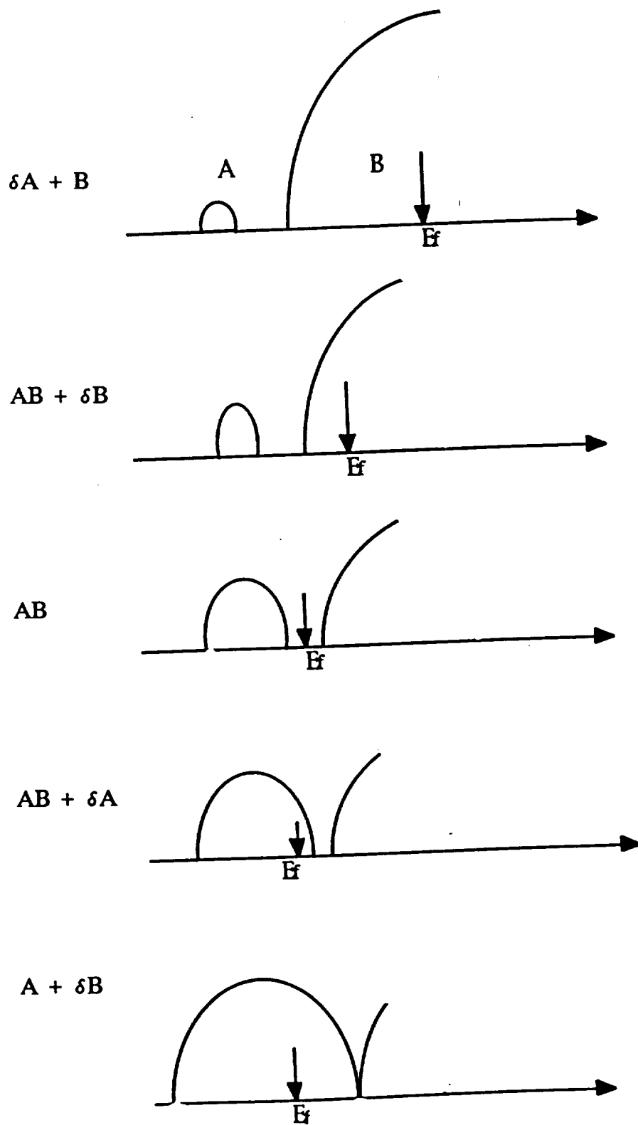
Figure 2.15 Schematical position of the Fermi level in the alloy.
